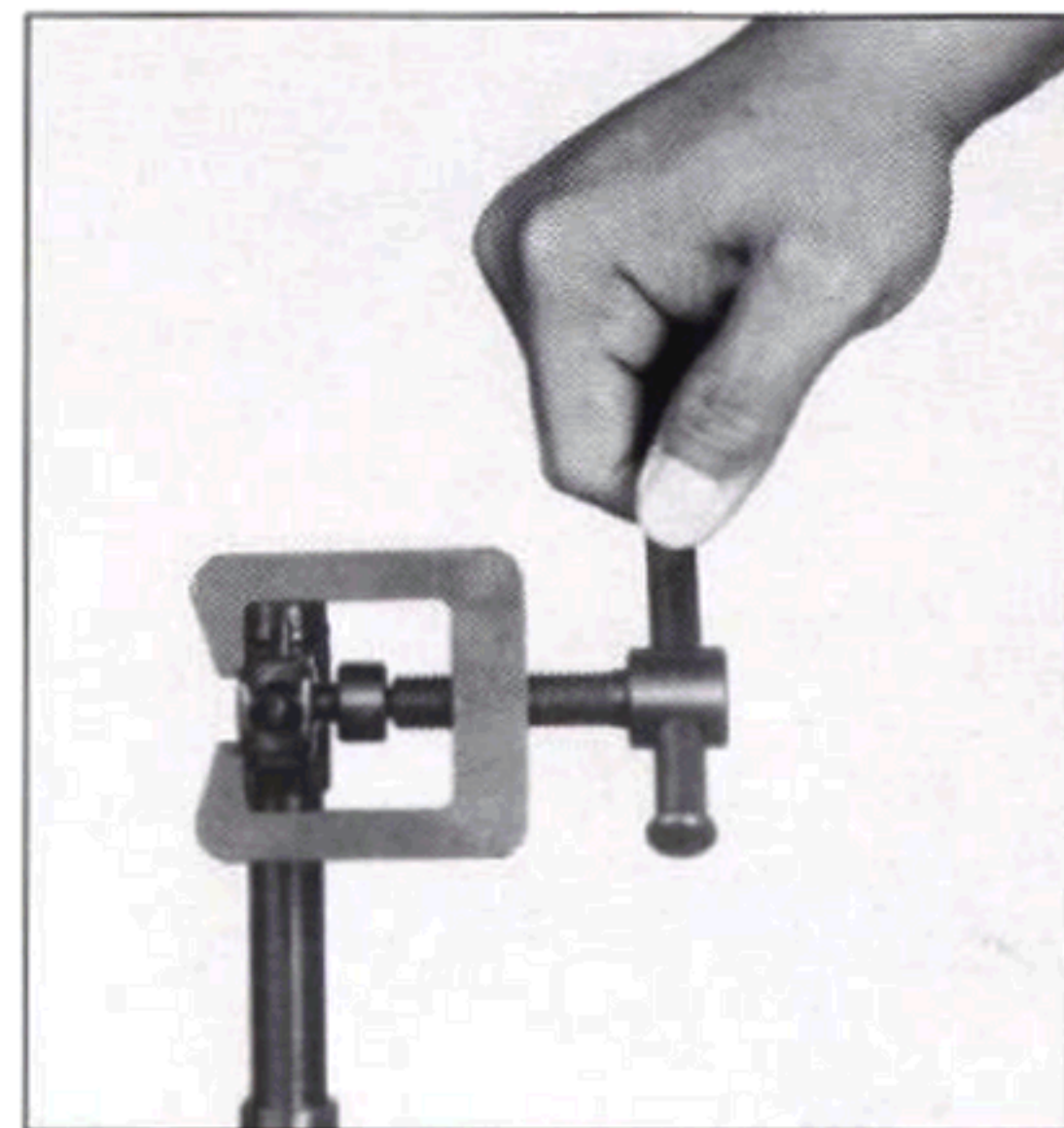
Fig. 23 Adjusting the front sight (windage) using the optional front sight adjustment tool.
