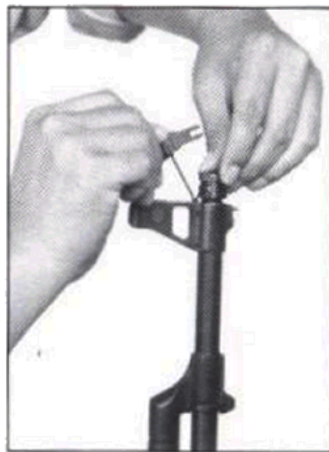
Fig. 32 Screwing the muzzle nut off while depressing the plunger.
