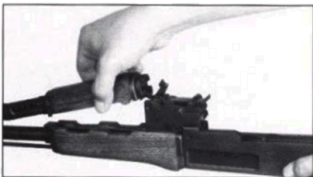
Fig. 30 Lifting the handguard/piston tube off.
