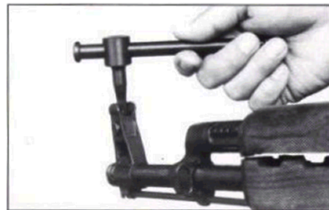
Fig. 22 Adjusting the front sight (elevation) using the optional front sight adjustment tool.
