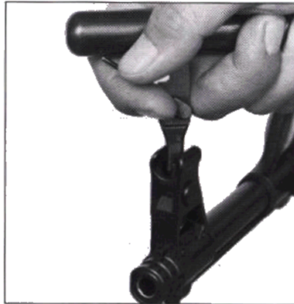
Fig. 21 Using the combination tool to adjust front sight (elevation).
