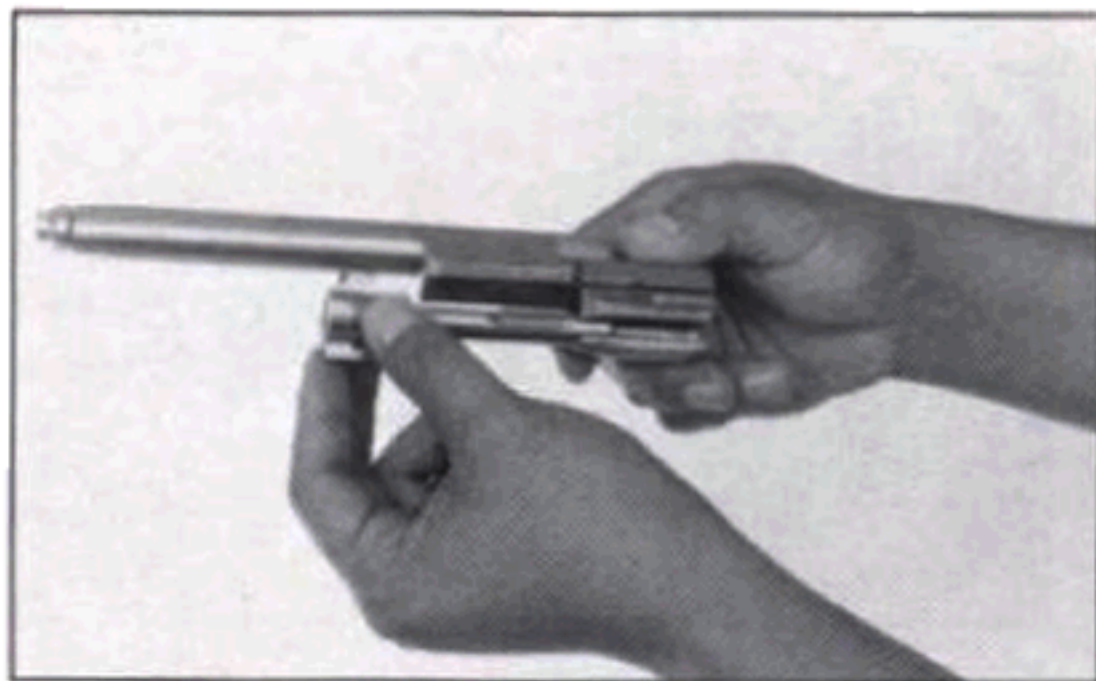
Fig. 29 Separating the bolt from the bolt carrier.
