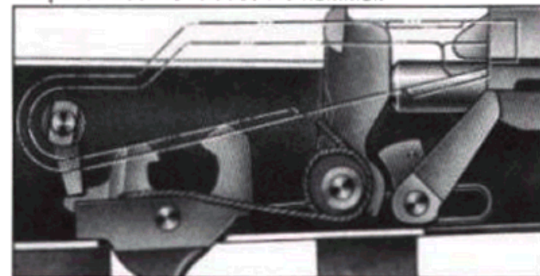
Fig. 5 The mechanism shown with the hammer down and the safety lever placed on "SAFE."
