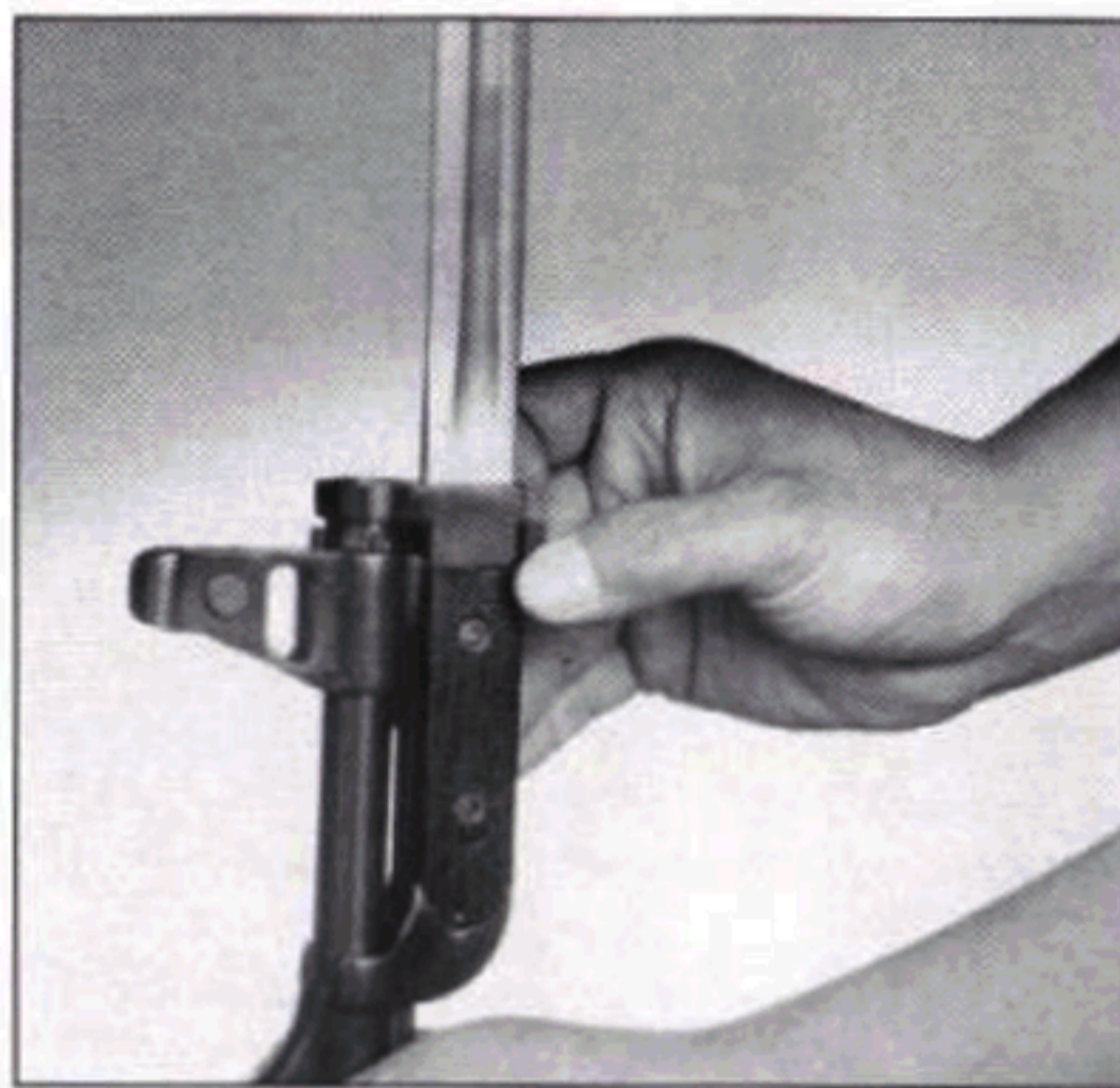
Fig. 17 Removing the bayonet.
