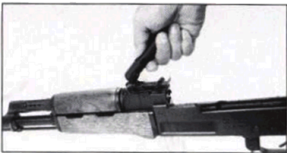
Fig. 31 Using the accessory tube to lift up the piston tube lock lever.
